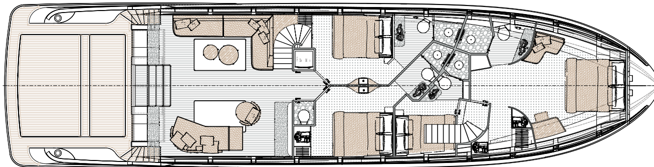
Main Deck
